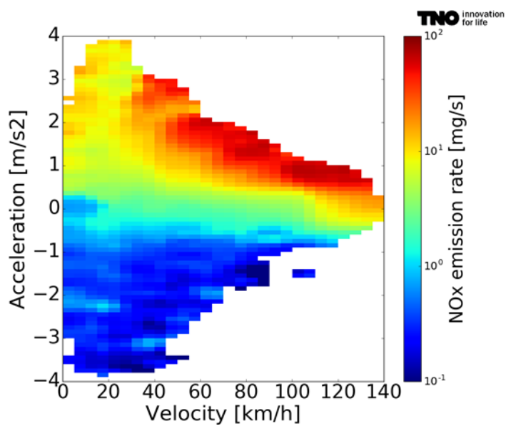
Figure 3-3: NO x emission rate [mg/s] of a Peugeot Partner Euro 6 diesel in bins of velocity and acceleration.
