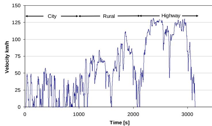
Figure 4: CADC (Common Artemis Driving Cycle)
