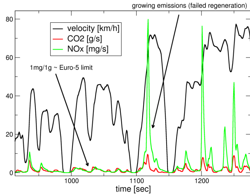
Figure 24 During rural driving NO x emissions may grow occasionally due to the delayed or failed regeneration of the trap.
