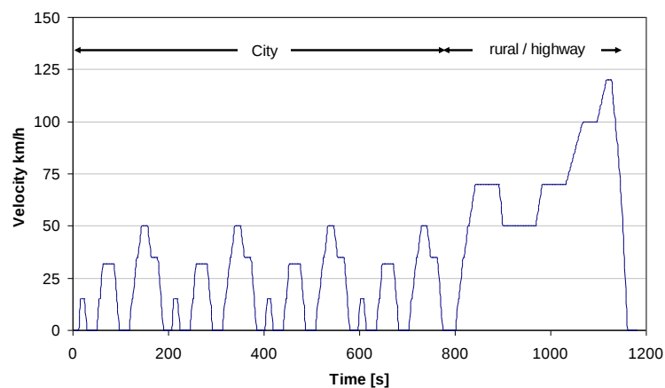
Figure 3: NEDC (New European Driving Cycle)
